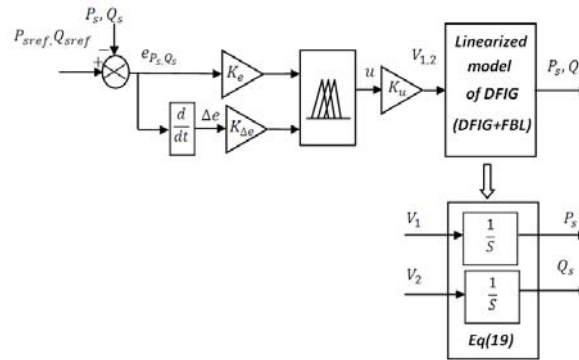
Figure 5. DFIG control scheme using proposed fuzzy-feedback linearization control (PFBL)
