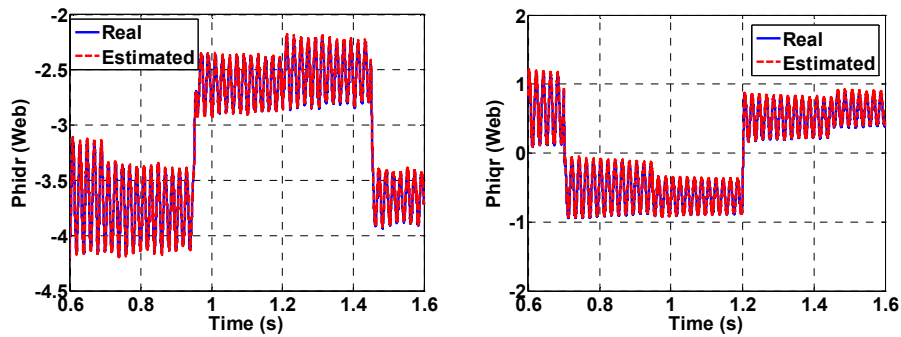
Figure 10. Direct and quadrature flux
